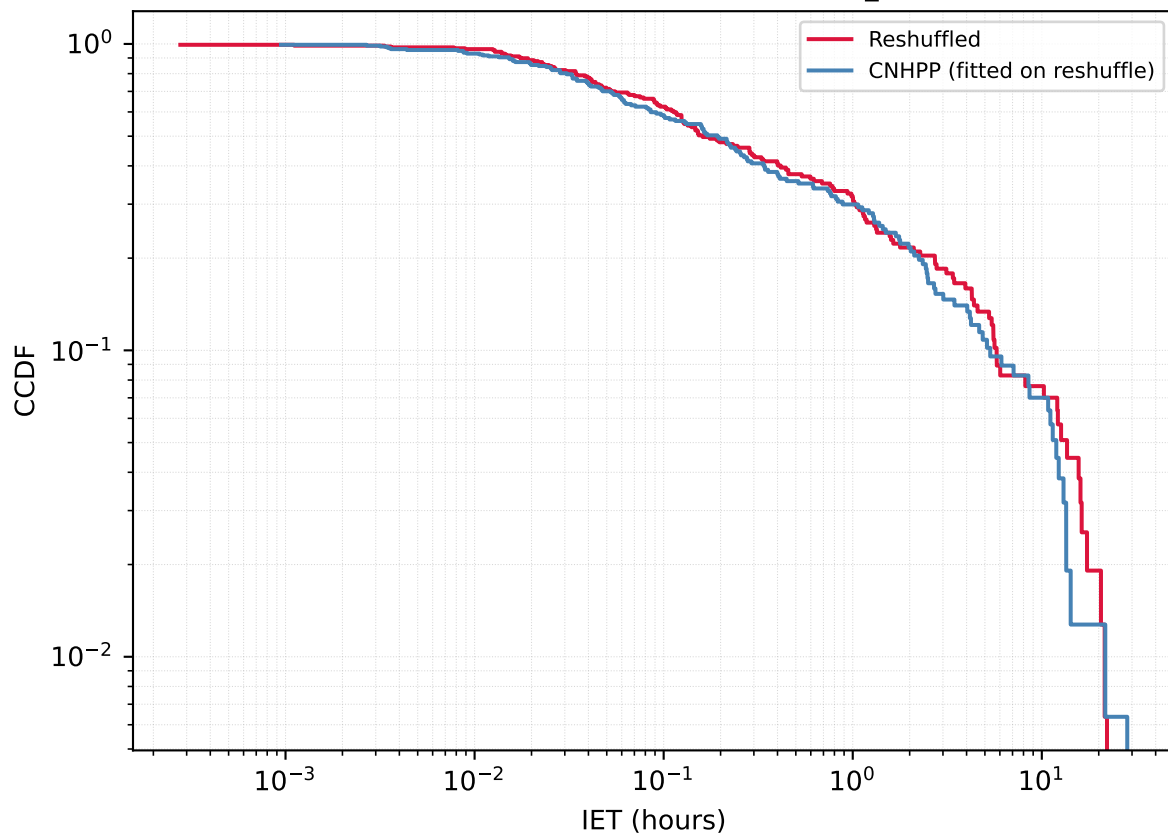
User 5212333848 - Reshuffled vs CNHPP A_{\text{fit}}=0.2897
